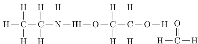
Ethanamine
